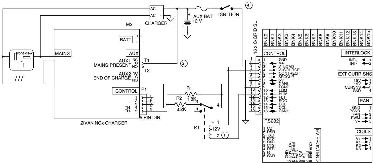
ELITHION BMS CONTROLLER
