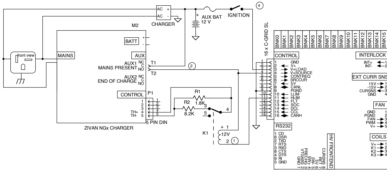
ELITHION BMS CONTROLLER
