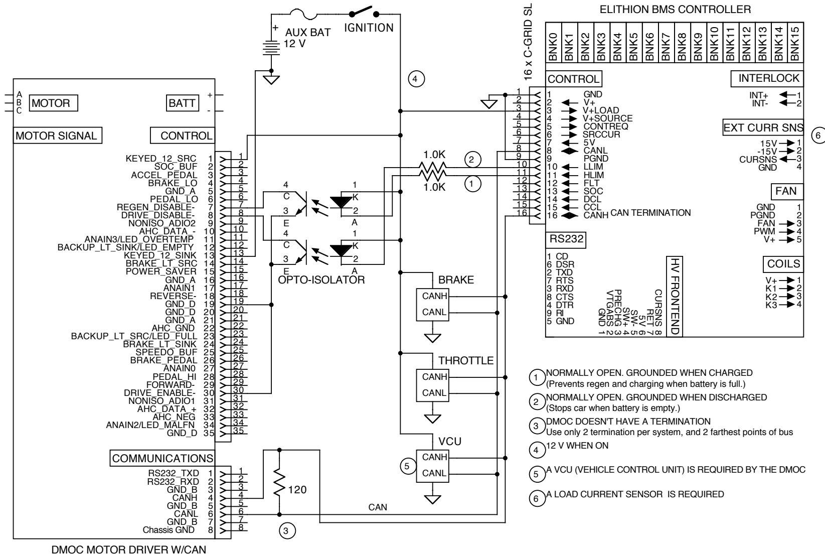
DMOC MOTOR DRIVER W/CAN
